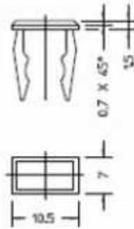
Lens dimensions
