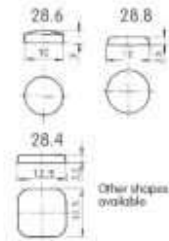
Lens dimensions
